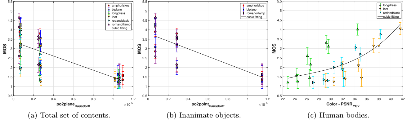
Figure 11. Best performing point-based metric on UNB subjective scores.
